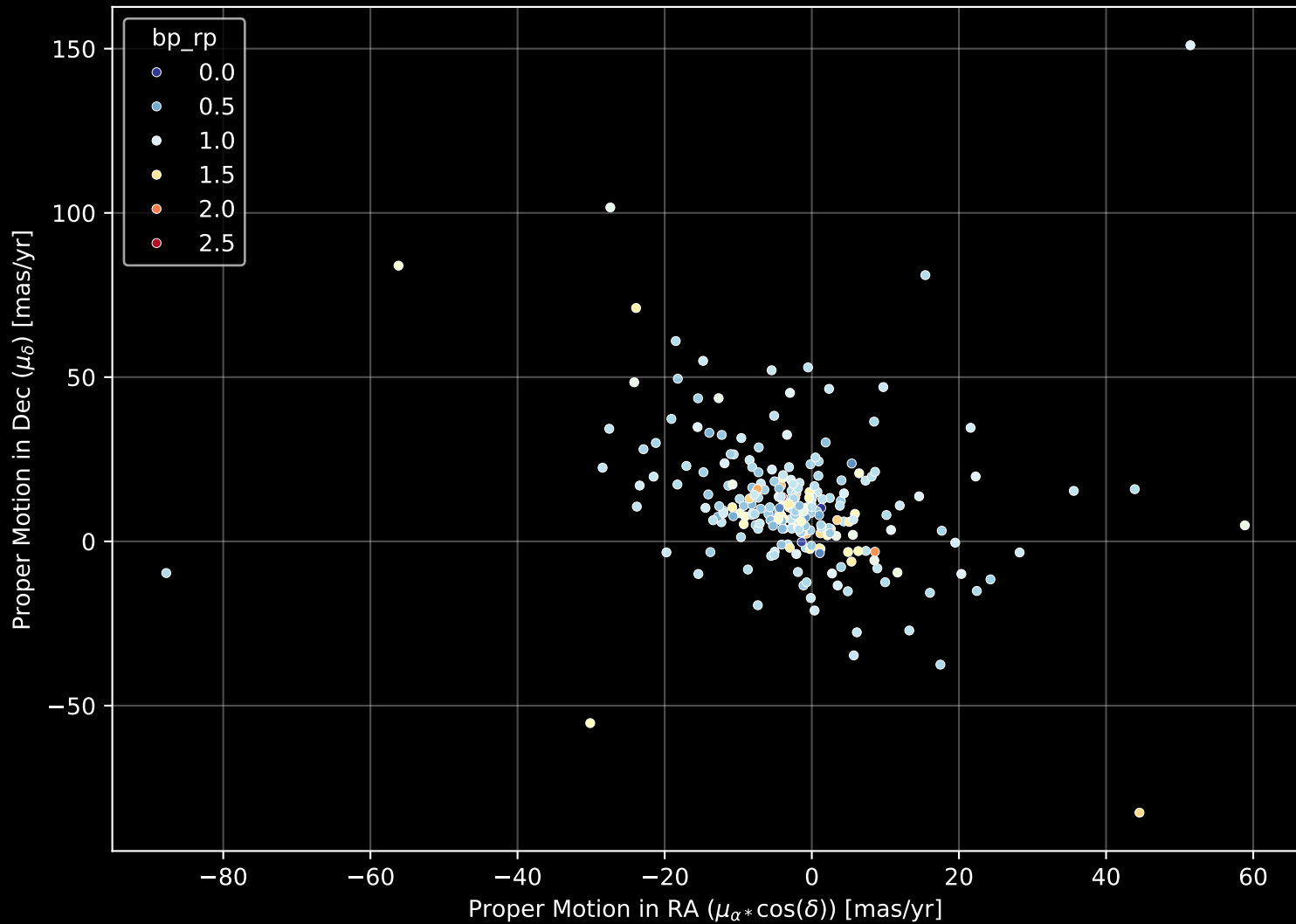
GALAH DR4 Field: [7165] Proper Motion Diagram (n= 252)
