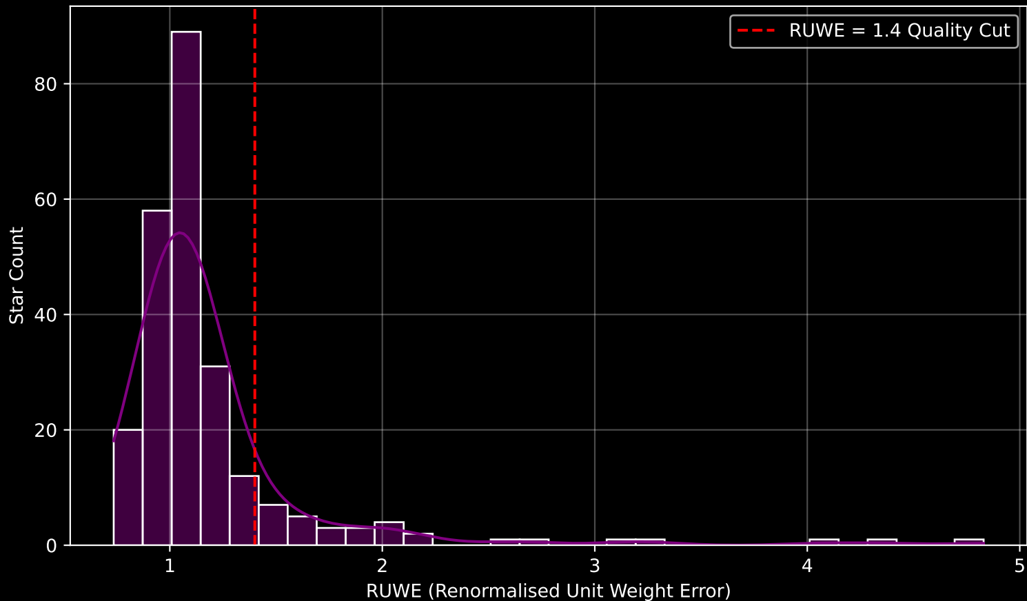
GALAH DR4 Field [7165] RUWE Distribution (n= 241)
