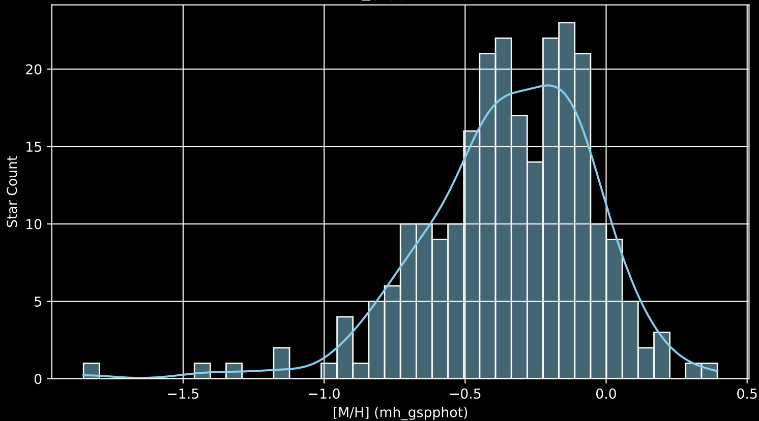
GALAH DR4 Field: [7165] [M/H] (mh_gspphot) (n= 248)
