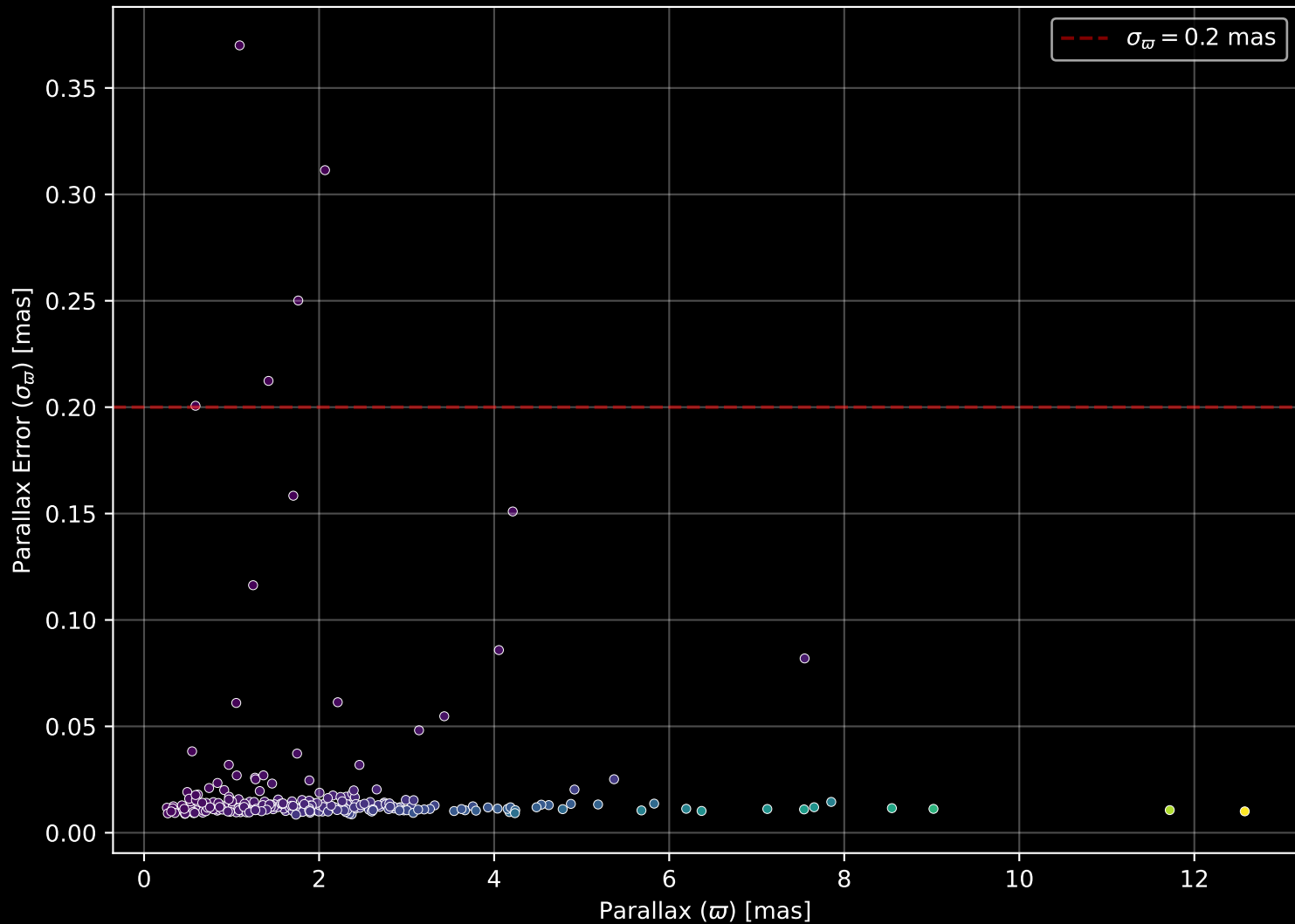
GALAH DR4 Field: [7165] Parallax Quality (n= 252)
