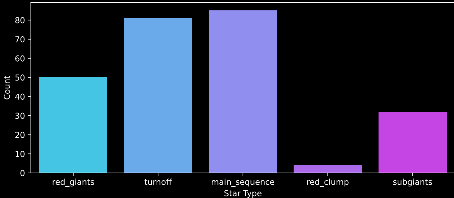
GALAH DR4 Field: [7165] Count plot of Star Type
